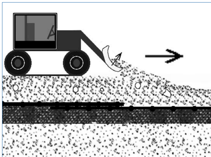
Figure 1: Geogrid overlapping and fill spread direction
